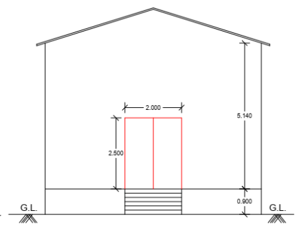
ELEVATION SCALE - 1:100
